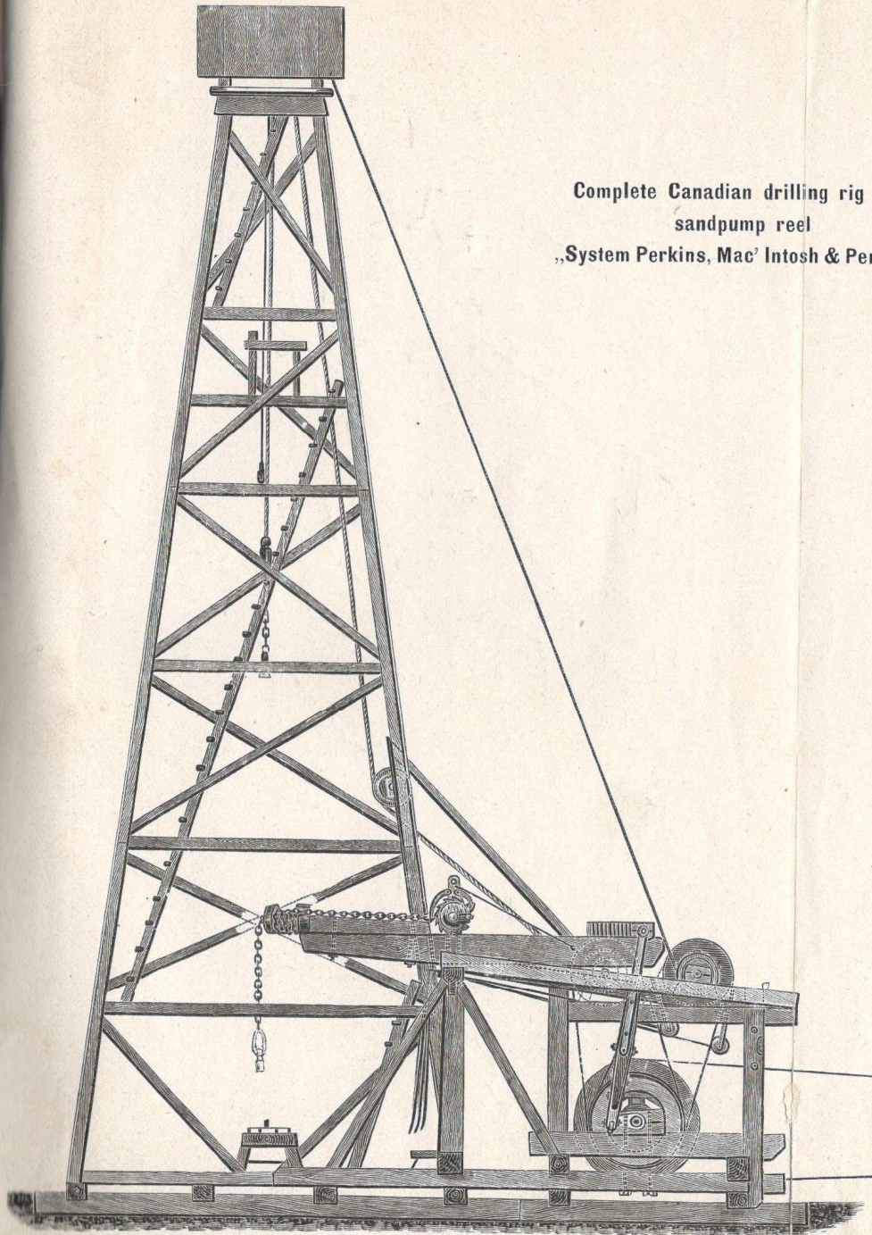
Side view.
